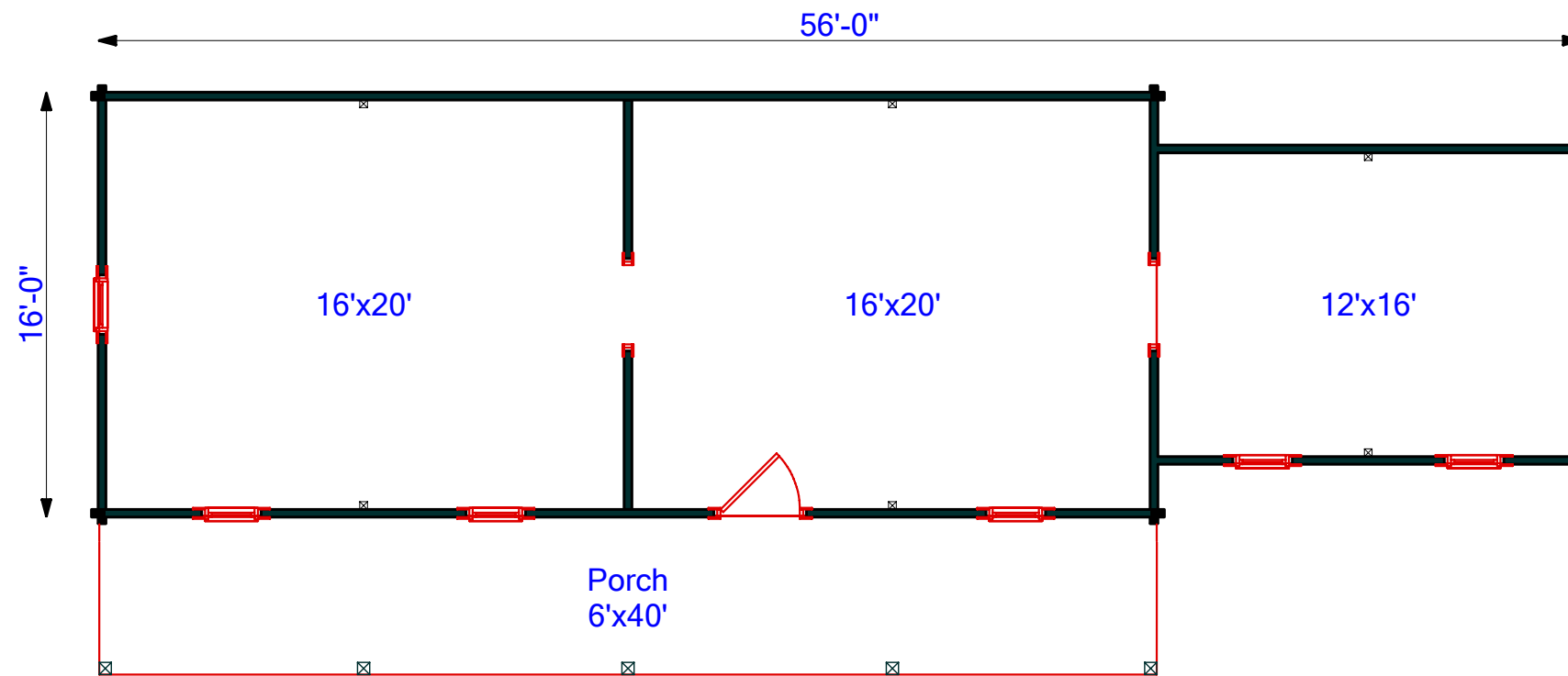
Floor Plan
